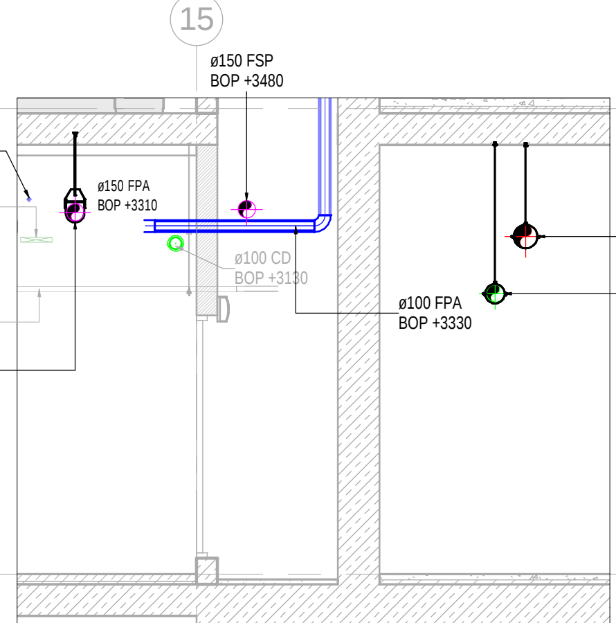
SECTION-FI SCALE : 1:50
