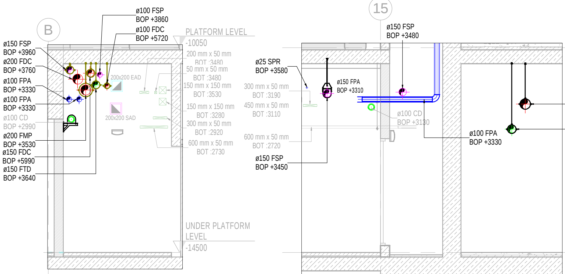
SECTION-FH SCALE : 1:50
