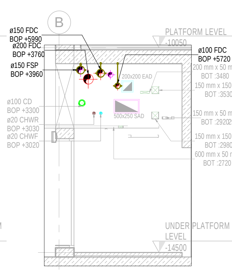
SECTION-FJ SCALE : 1:50
